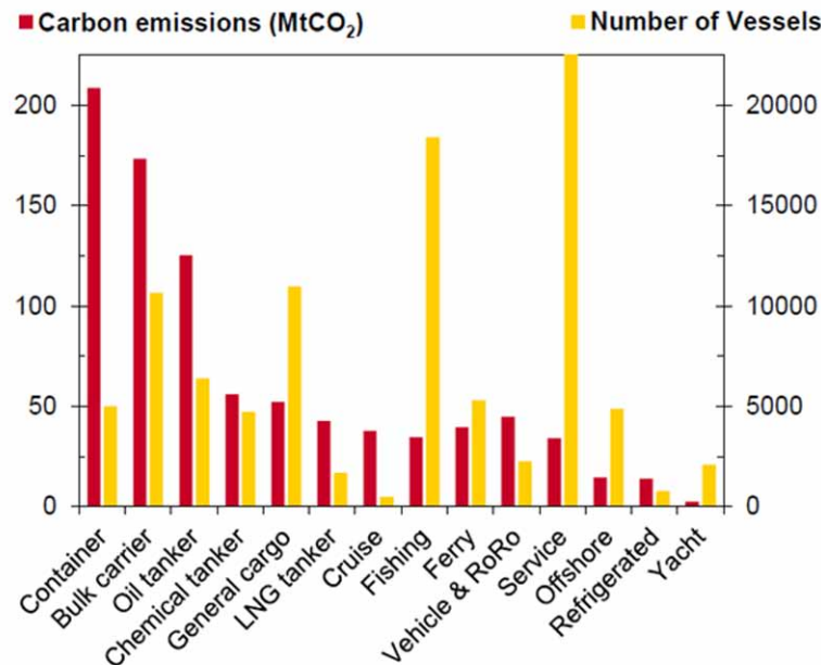
Figure 1. Number of ships and their carbon emissions by category in 2017 (Source: Balcombe et al. (2019))
