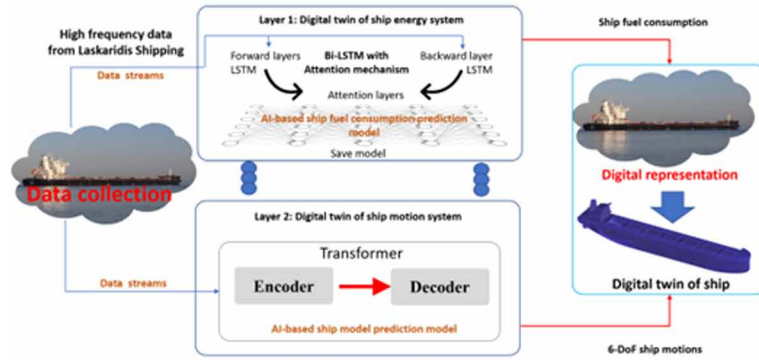
Figure 2. The overall procedure of AI-based ship digital twin
