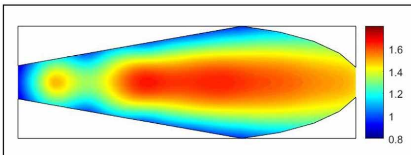
Figure 13. Fuel-Air equivalence ratio distribution in the jet area 5deg CA after injection, 50% load, B30
