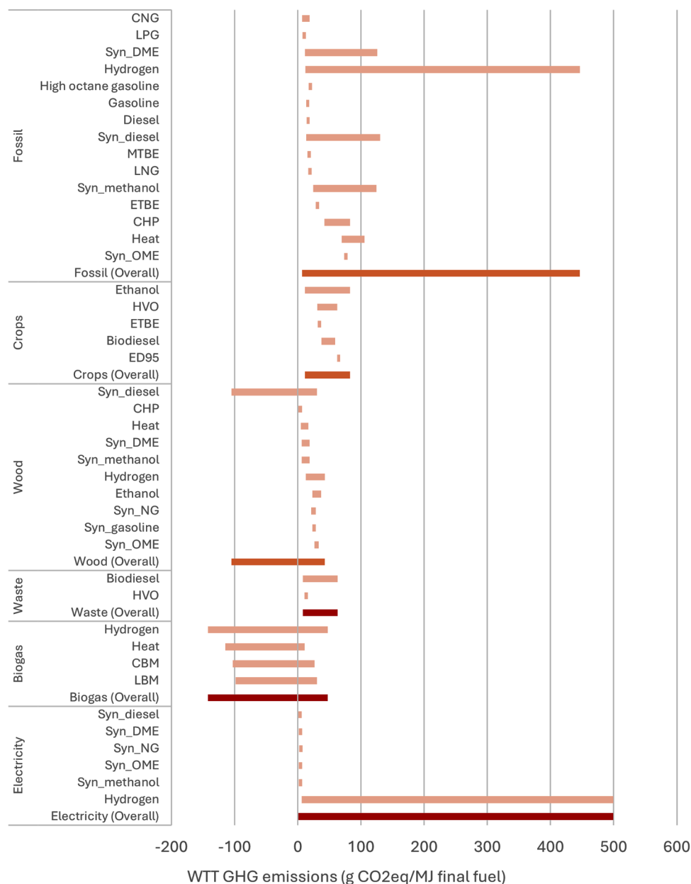
Figure 1. WTT GHG missions of various fuel production pathways
