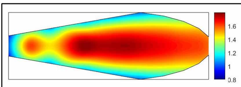
Figure 14. Fuel-Air equivalence ratio distribution in the jet area 5deg CA after injection, Low O_2 HFO
