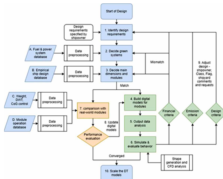
Figure 2. Proposed DT-based design process
